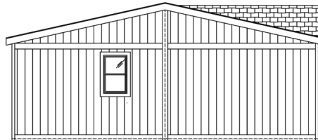
REAR ENDWALL
